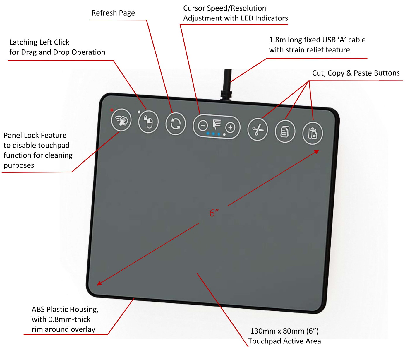
Figure 2: Touchpad Features
